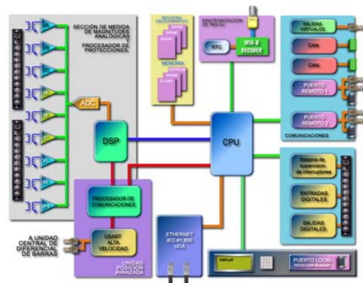
Figure 1 . Bay IED block diagram
